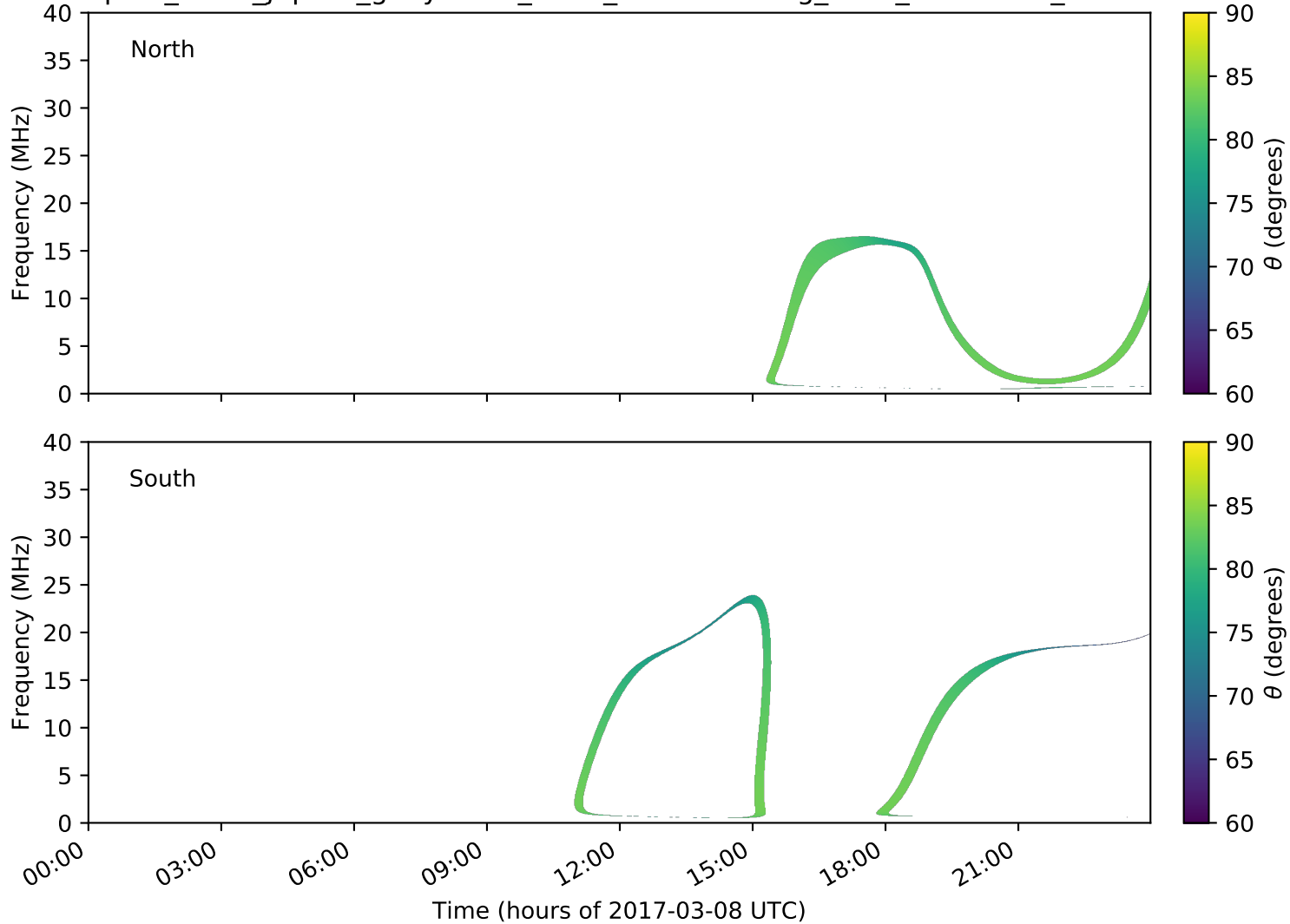
expres_earth_jupiter_ganymede_isaac_lossc-wid1deg_3kev_20170308_v01.cdf
