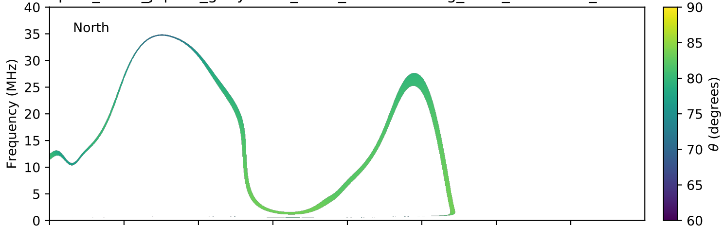
expres_earth_jupiter_ganymede_isaac_lossc-wid1deg_3kev_20170304_v01.cdf
