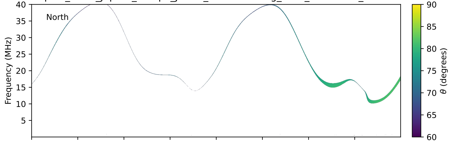
expres_earth_jupiter_europa_jrm33_lossc-wid1deg_3kev_20170323_v11.cdf
