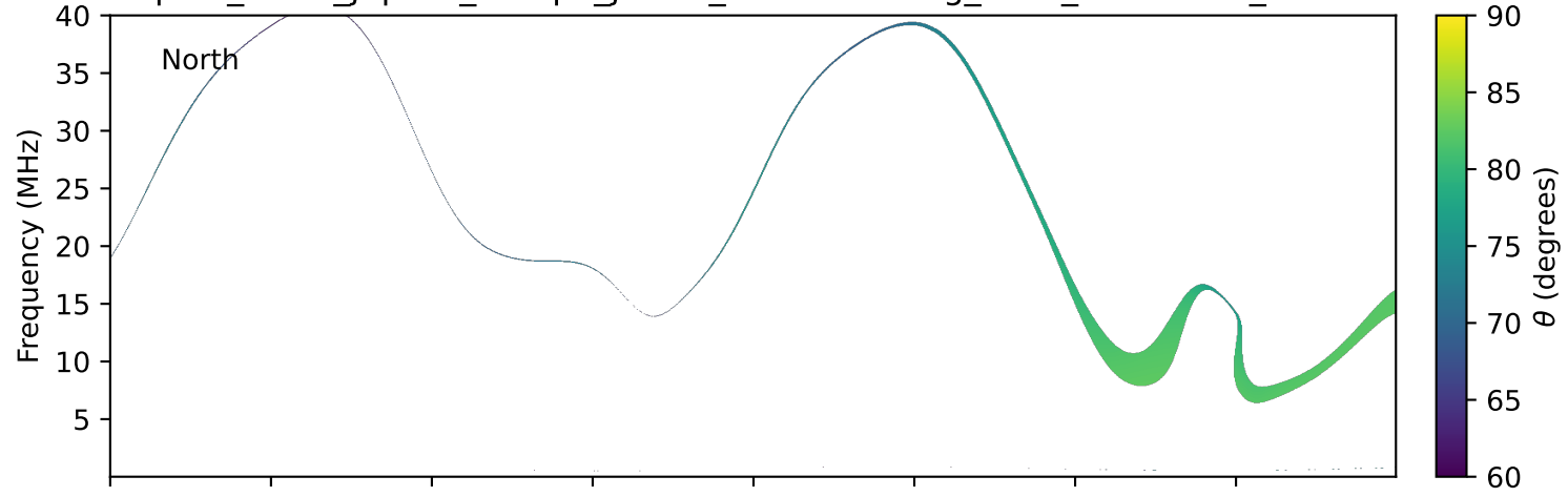
expres_earth_jupiter_europa_jrm33_lossc-wid1deg_3kev_20170316_v11.cdf
