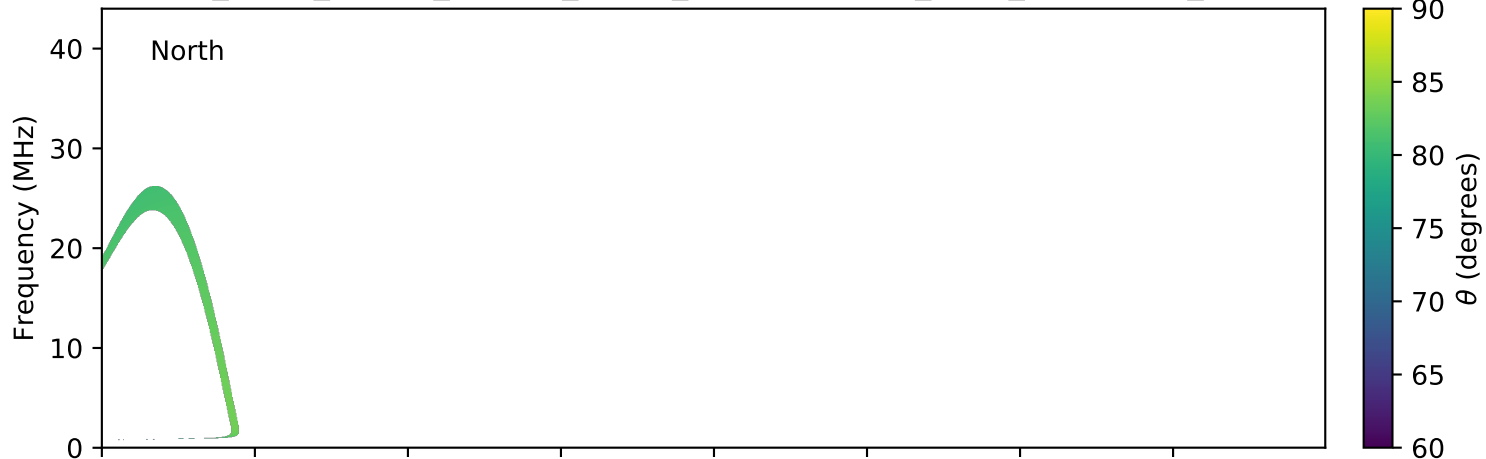
expres_earth_jupiter_europa_jrm09_lossc-wid1deg_3kev_20170324_v01.cdf
