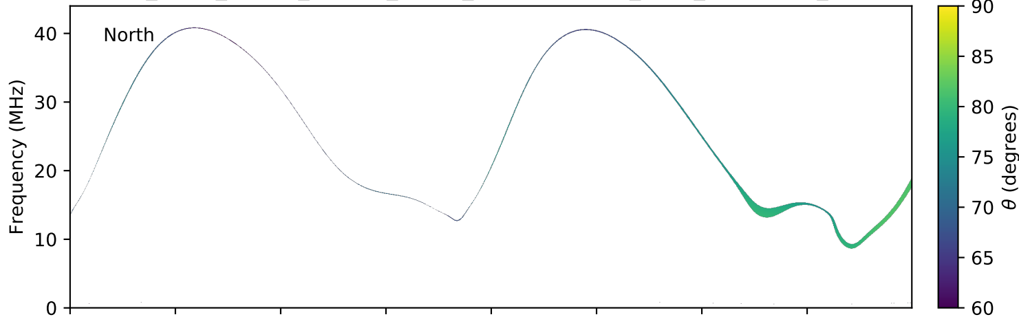
expres_earth_jupiter_europa_jrm09_lossc-wid1deg_3kev_20170323_v01.cdf
