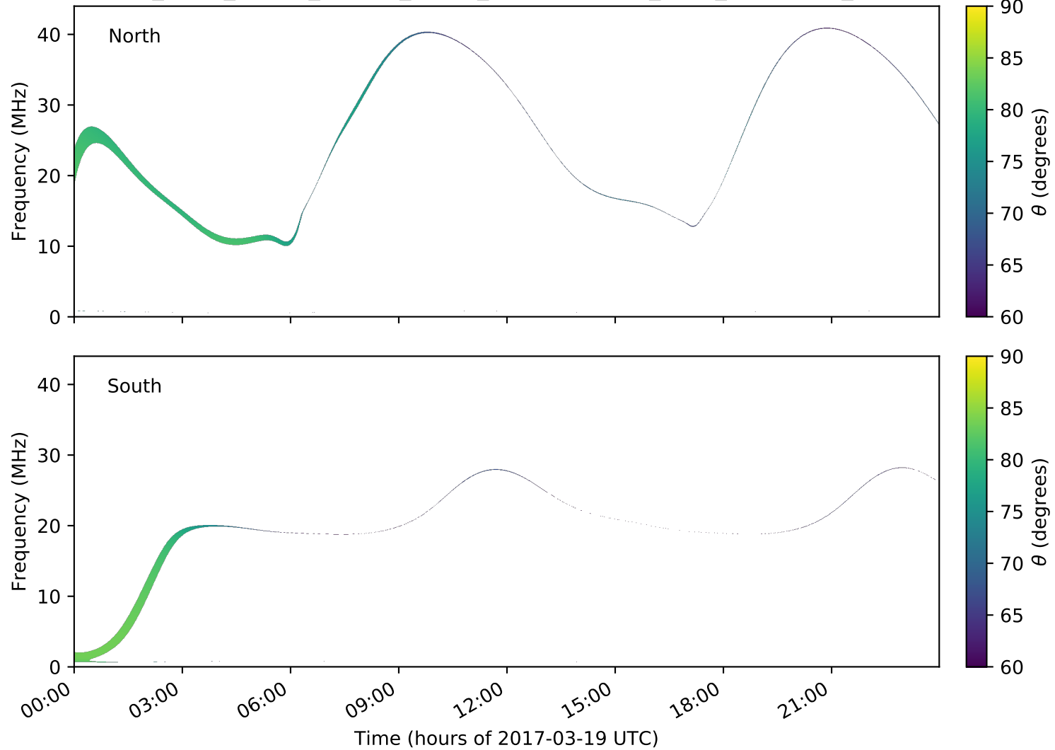
expres_earth_jupiter_europa_jrm09_lossc-wid1deg_3kev_20170319_v01.cdf
