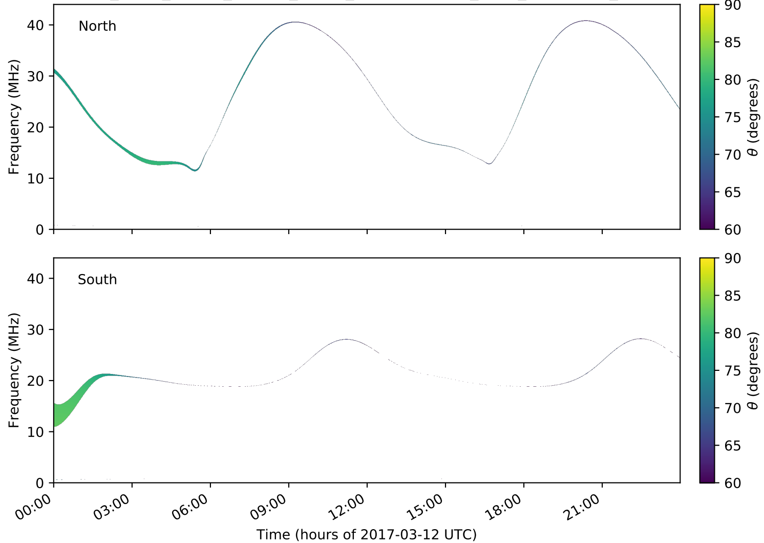
expres_earth_jupiter_europa_jrm09_lossc-wid1deg_3kev_20170312_v01.cdf
