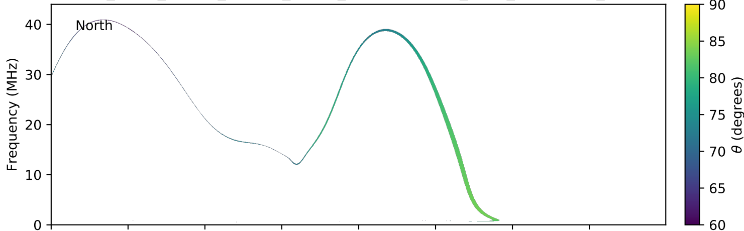
expres_earth_jupiter_europa_jrm09_lossc-wid1deg_3kev_20170302_v01.cdf
