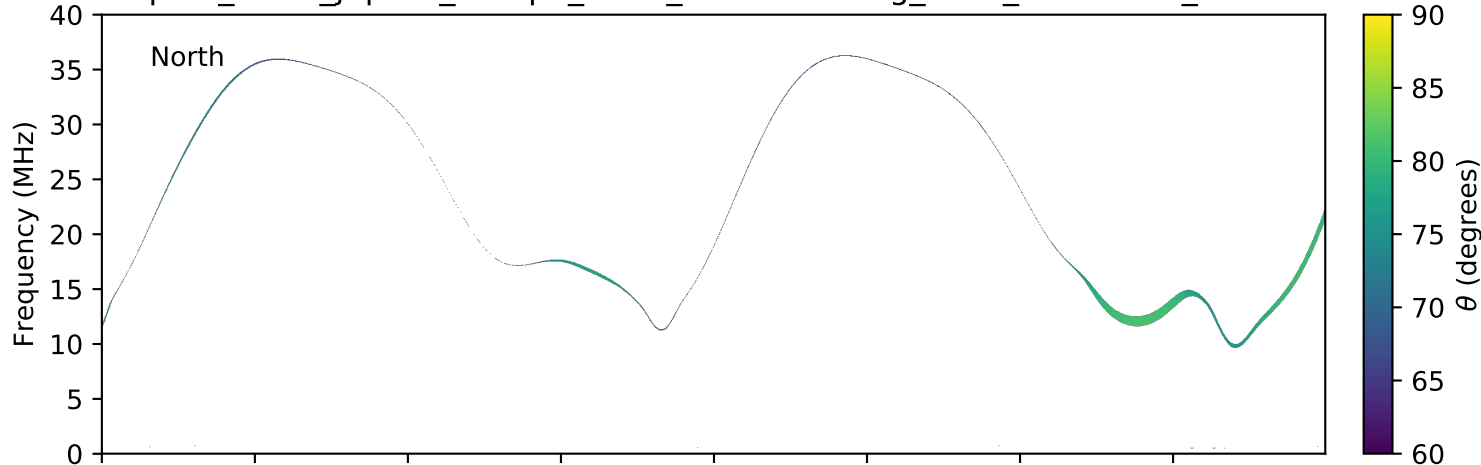
expres_earth_jupiter_europa_isaac_lossc-wid1deg_3kev_20170330_v01.cdf
