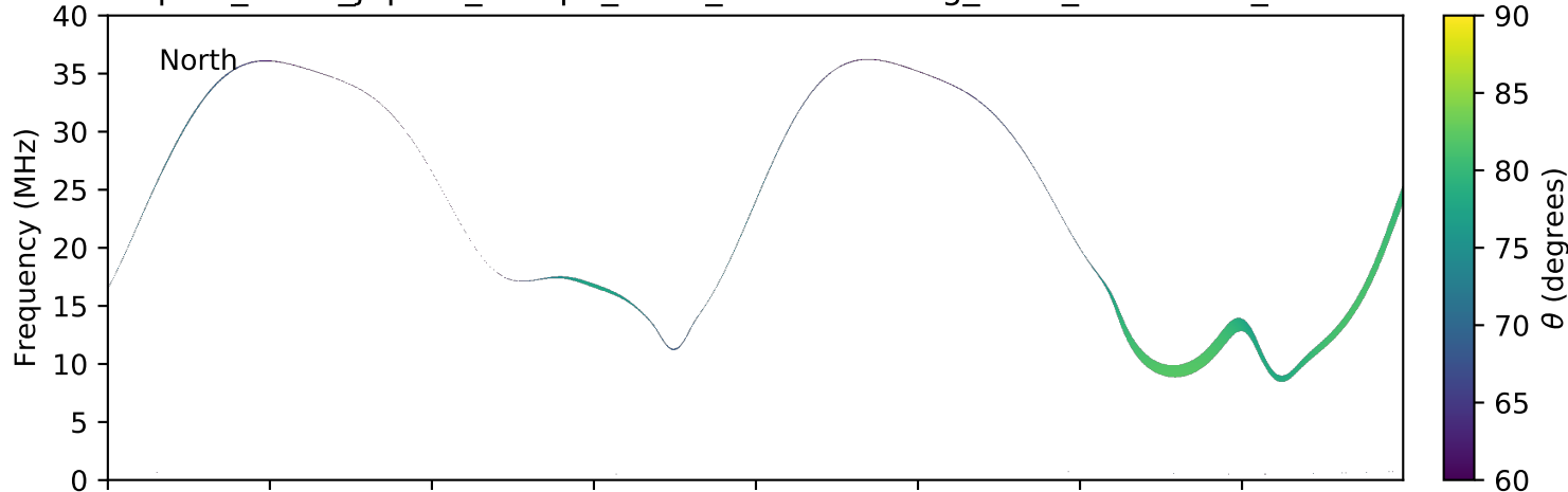
expres_earth_jupiter_europa_isaac_lossc-wid1deg_3kev_20170323_v01.cdf
