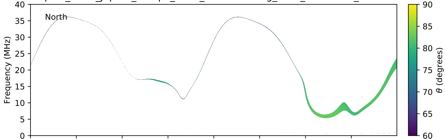
expres_earth_jupiter_europa_isaac_lossc-wid1deg_3kev_20170316_v01.cdf
