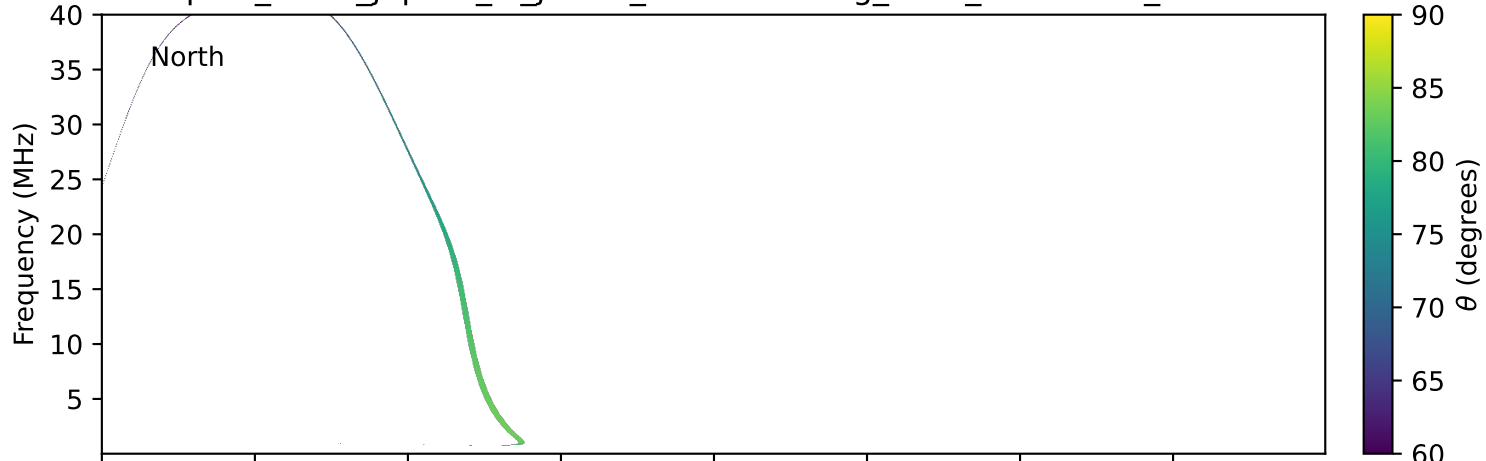
expres_earth_jupiter_io_jrm33_lossc-wid1deg_3kev_20170218_v11.cdf
