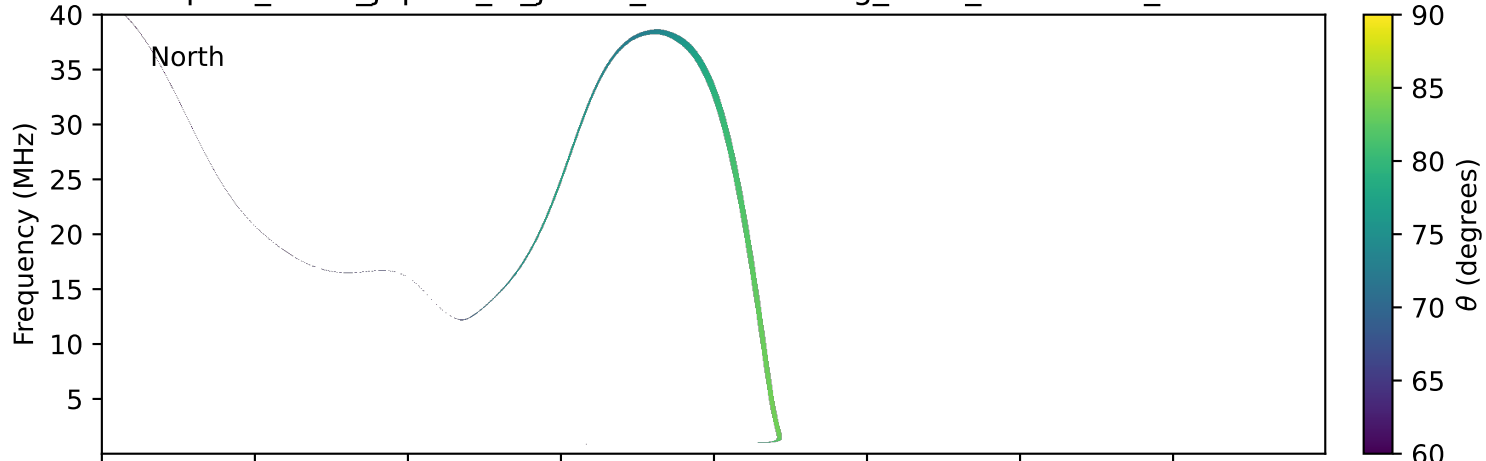
expres_earth_jupiter_io_jrm33_lossc-wid1deg_3kev_20170209_v11.cdf
