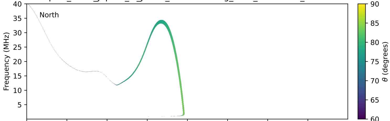
expres_earth_jupiter_io_jrm33_lossc-wid1deg_3kev_20170202_v11.cdf
