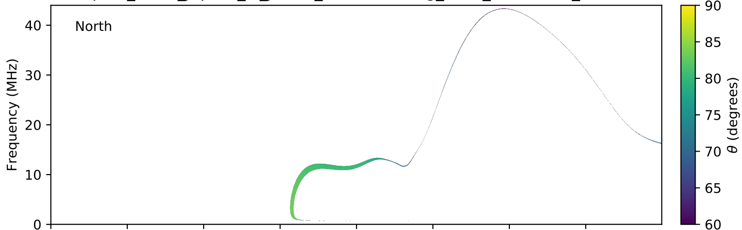
expres_earth_jupiter_io_jrm09_lossc-wid1deg_3kev_20170226_v01.cdf
