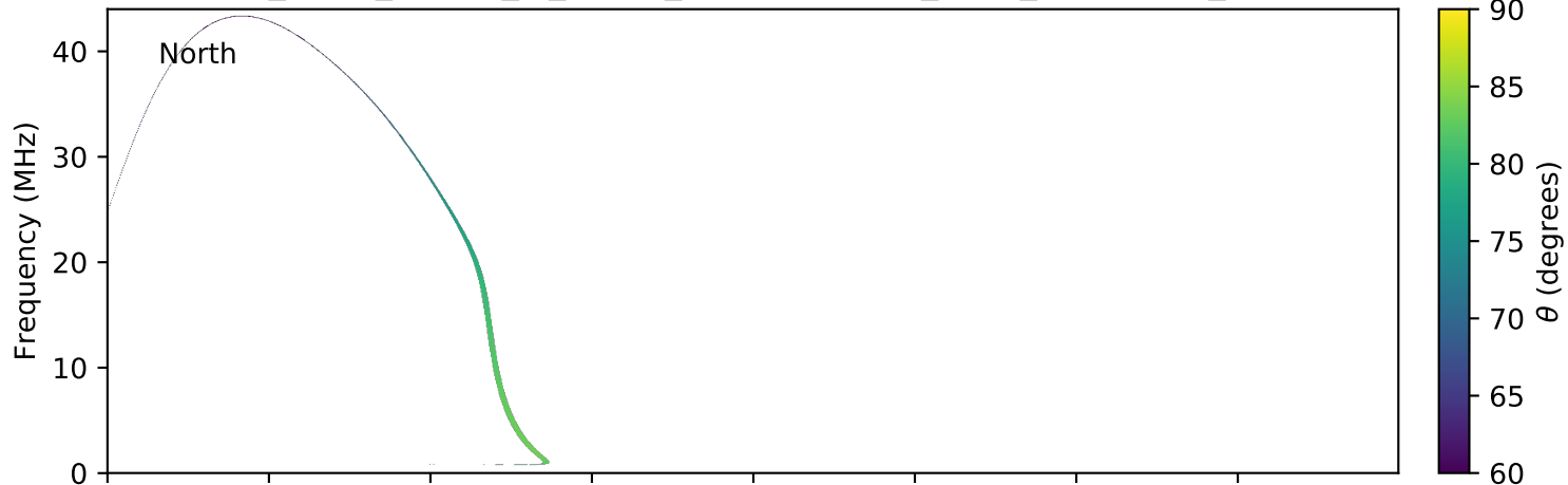
expres_earth_jupiter_io_jrm09_lossc-wid1deg_3kev_20170218_v01.cdf
