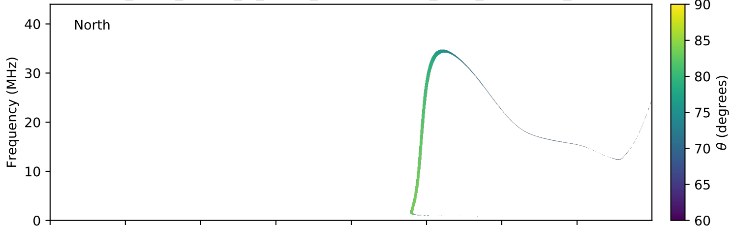
expres_earth_jupiter_io_jrm09_lossc-wid1deg_3kev_20170217_v01.cdf
