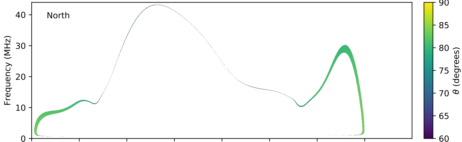
expres_earth_jupiter_io_jrm09_lossc-wid1deg_3kev_20170214_v01.cdf
