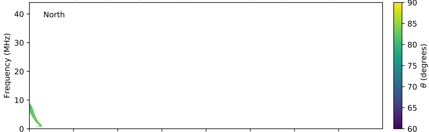
expres_earth_jupiter_io_jrm09_lossc-wid1deg_3kev_20170213_v01.cdf
