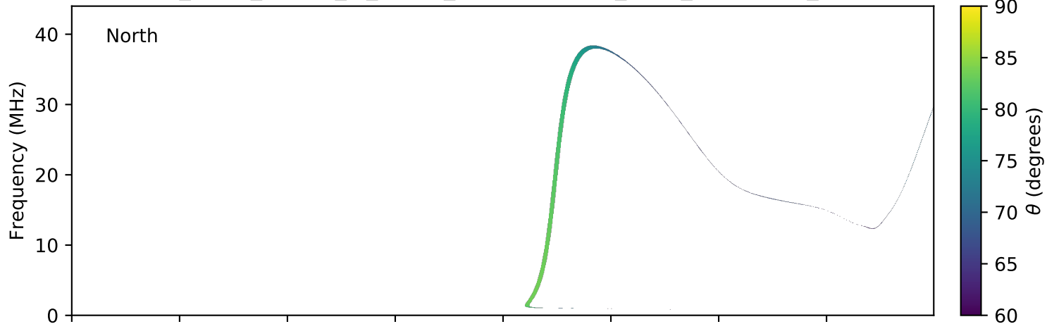
expres_earth_jupiter_io_jrm09_lossc-wid1deg_3kev_20170210_v01.cdf
