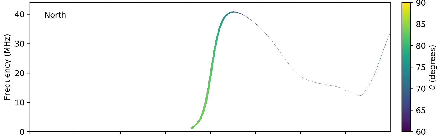
expres_earth_jupiter_io_jrm09_lossc-wid1deg_3kev_20170203_v01.cdf
