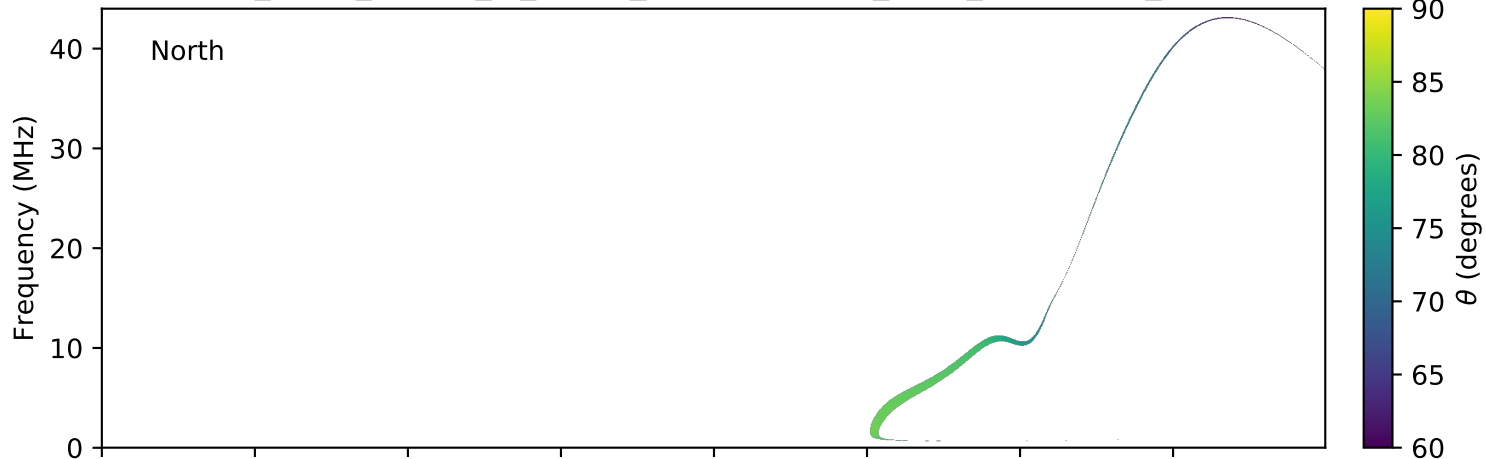
expres_earth_jupiter_io_jrm09_lossc-wid1deg_3kev_20170201_v01.cdf
