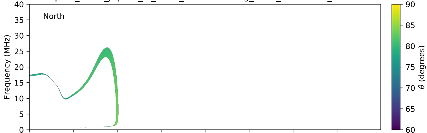
expres_earth_jupiter_io_isaac_lossc-wid1deg_3kev_20170227_v01.cdf
