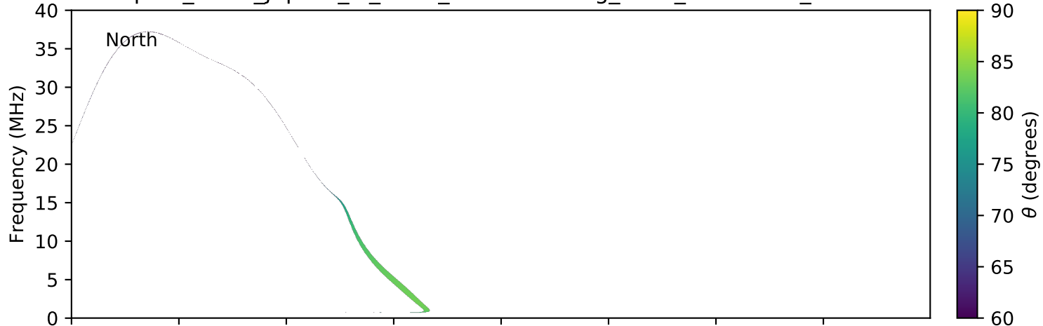
expres_earth_jupiter_io_isaac_lossc-wid1deg_3kev_20170225_v01.cdf
