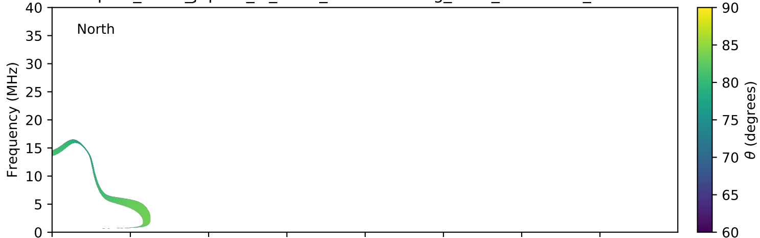
expres_earth_jupiter_io_isaac_lossc-wid1deg_3kev_20170220_v01.cdf
