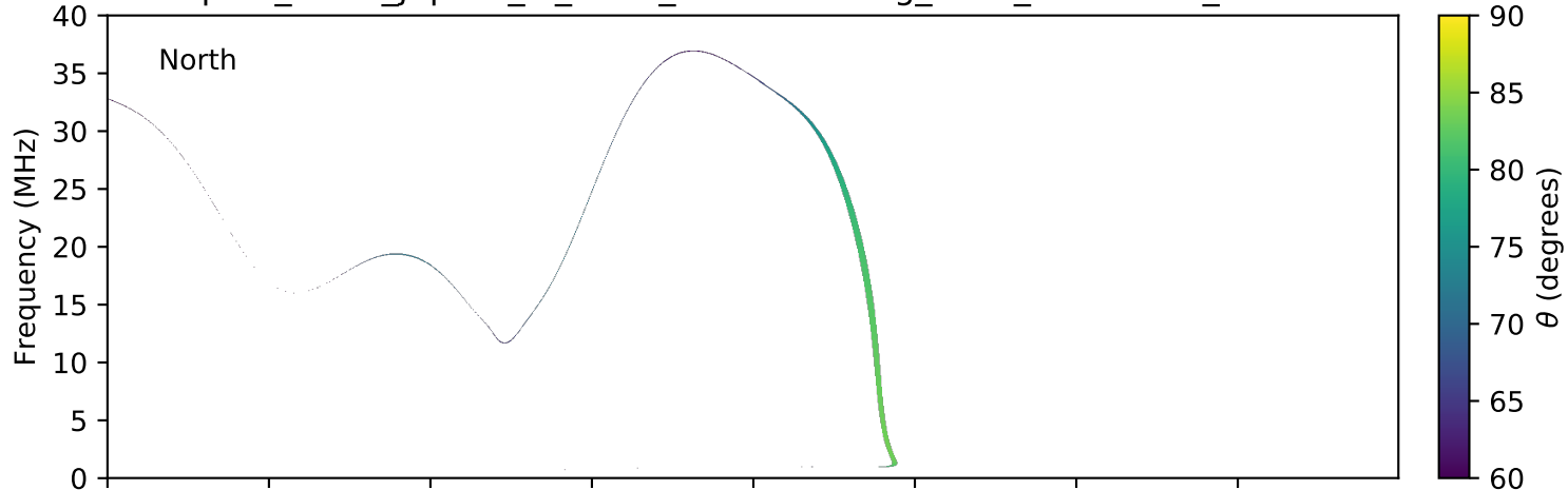
expres_earth_jupiter_io_isaac_lossc-wid1deg_3kev_20170216_v01.cdf
