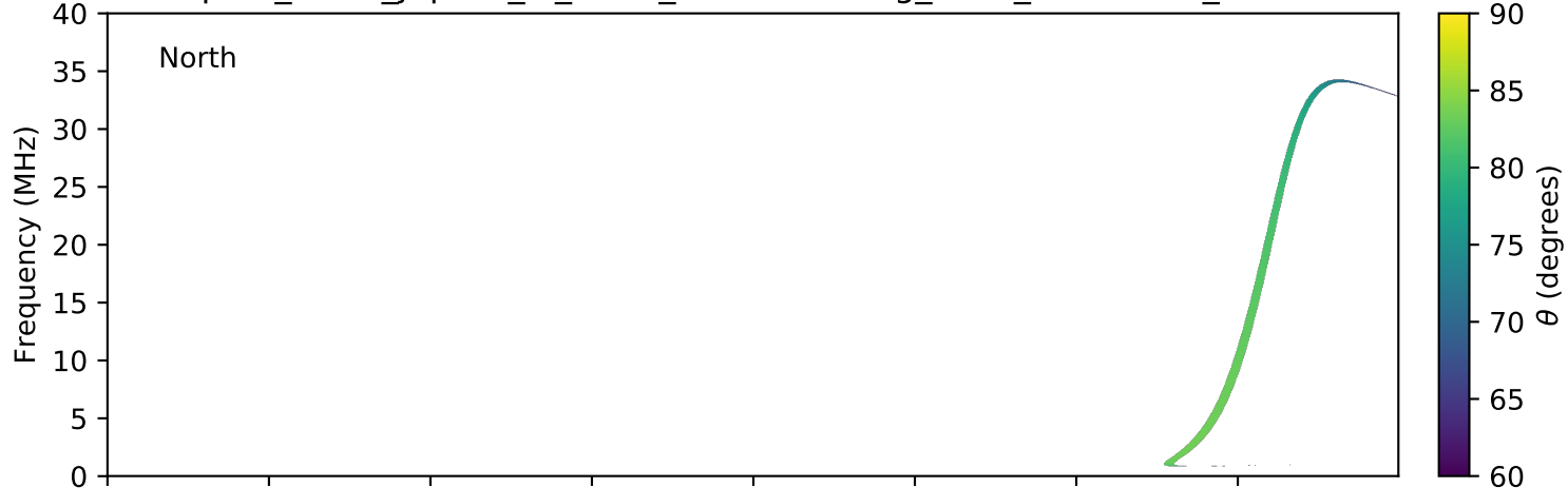
expres_earth_jupiter_io_isaac_lossc-wid1deg_3kev_20170215_v01.cdf
