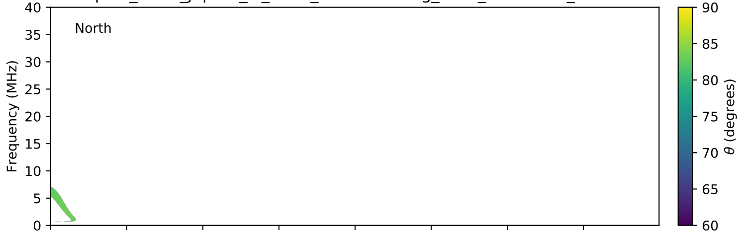
expres_earth_jupiter_io_isaac_lossc-wid1deg_3kev_20170213_v01.cdf
