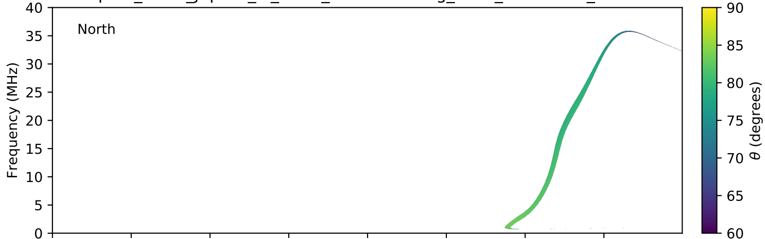
expres_earth_jupiter_io_isaac_lossc-wid1deg_3kev_20170208_v01.cdf
