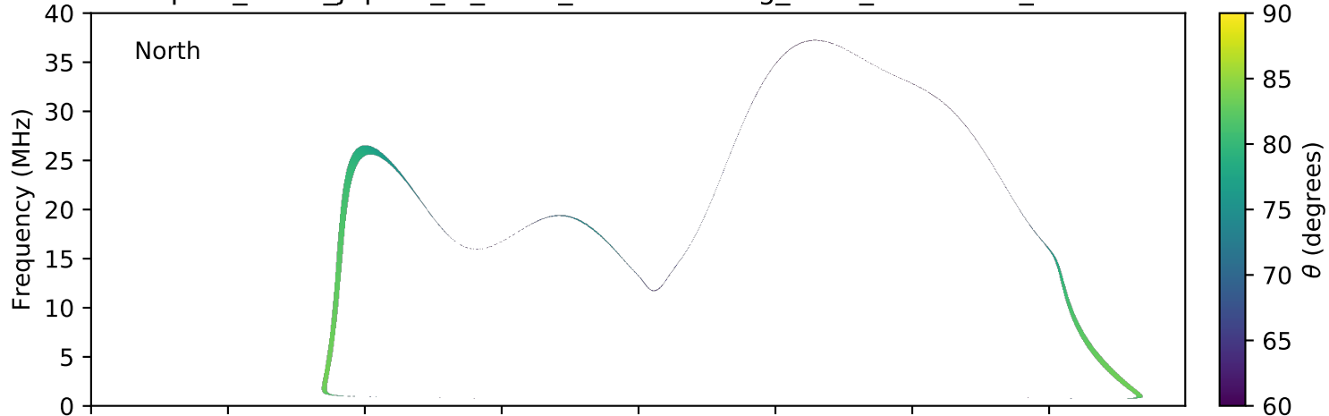
expres_earth_jupiter_io_isaac_lossc-wid1deg_3kev_20170205_v01.cdf
