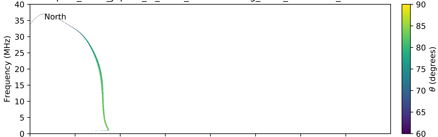
expres_earth_jupiter_io_isaac_lossc-wid1deg_3kev_20170204_v01.cdf
