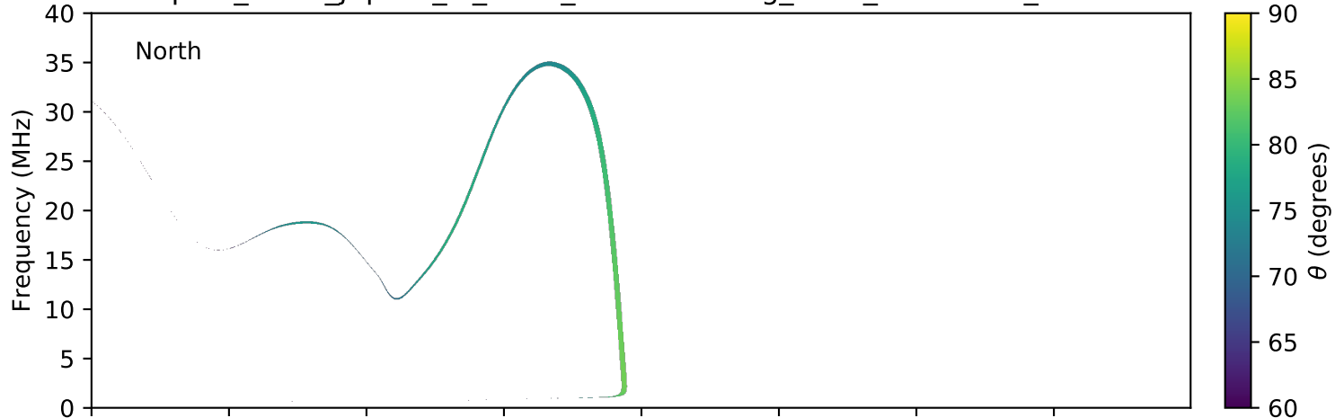
expres_earth_jupiter_io_isaac_lossc-wid1deg_3kev_20170202_v01.cdf
