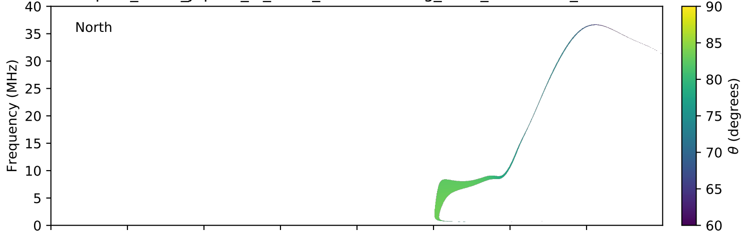
expres_earth_jupiter_io_isaac_lossc-wid1deg_3kev_20170201_v01.cdf
