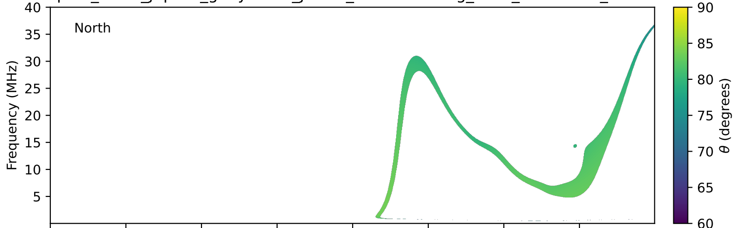
expres_earth_jupiter_ganymede_jrm33_lossc-wid1deg_3kev_20170222_v11.cdf
