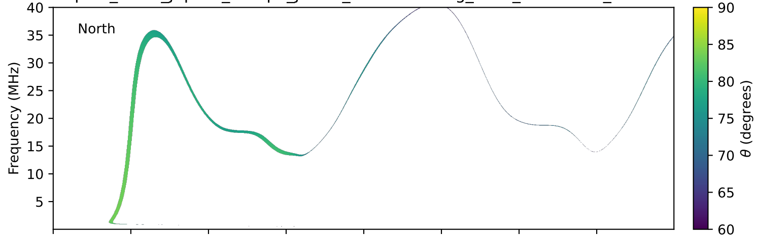
expres_earth_jupiter_europa_jrm33_lossc-wid1deg_3kev_20170215_v11.cdf
