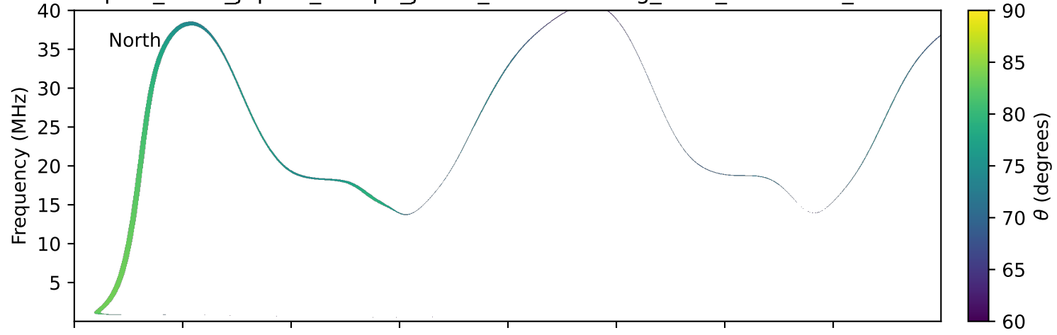
expres_earth_jupiter_europa_jrm33_lossc-wid1deg_3kev_20170208_v11.cdf
