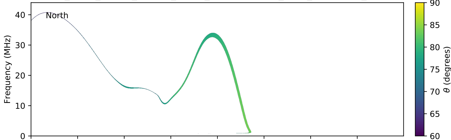
expres_earth_jupiter_europa_jrm09_lossc-wid1deg_3kev_20170216_v01.cdf
