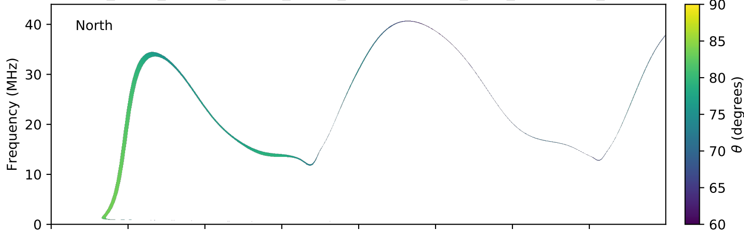
expres_earth_jupiter_europa_jrm09_lossc-wid1deg_3kev_20170215_v01.cdf
