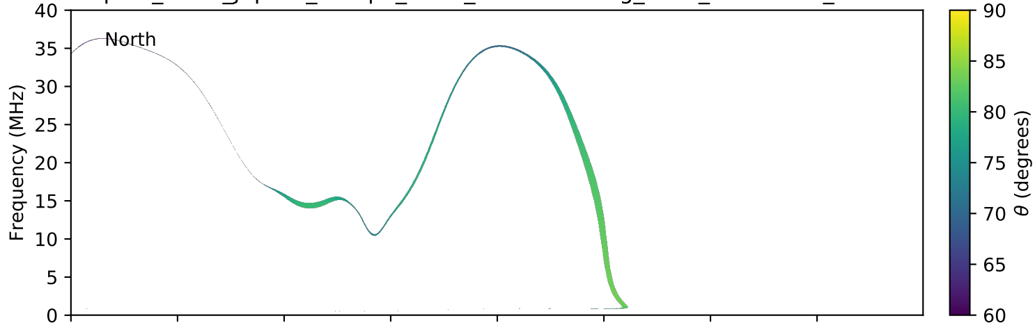
expres_earth_jupiter_europa_isaac_lossc-wid1deg_3kev_20170223_v01.cdf
