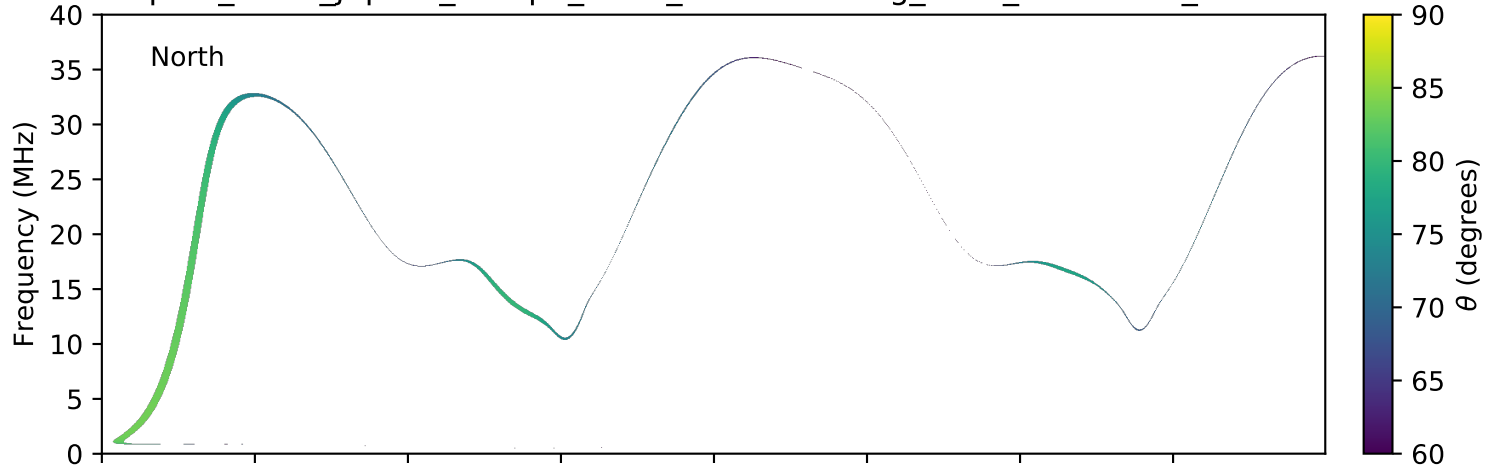
expres_earth_jupiter_europa_isaac_lossc-wid1deg_3kev_20170208_v01.cdf
