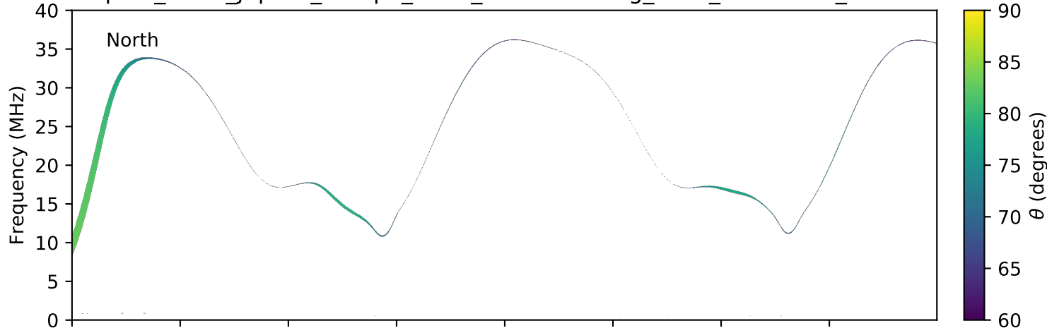
expres_earth_jupiter_europa_isaac_lossc-wid1deg_3kev_20170201_v01.cdf
