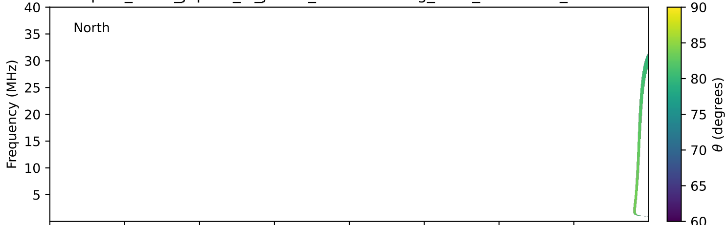
expres_earth_jupiter_io_jrm33_lossc-wid1deg_3kev_20161222_v11.cdf
