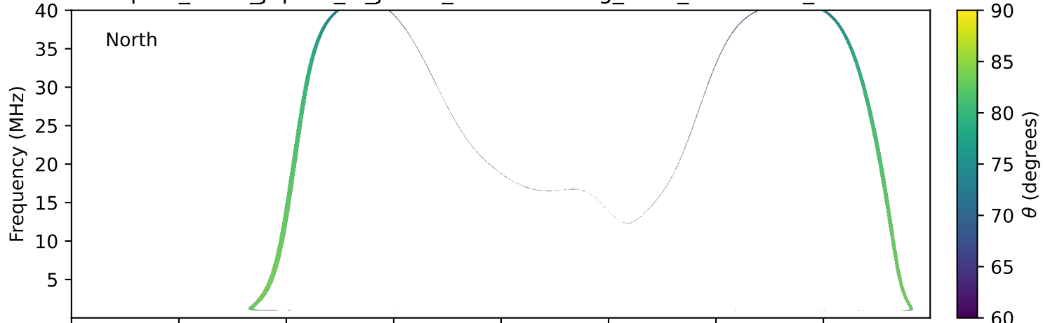
expres_earth_jupiter_io_jrm33_lossc-wid1deg_3kev_20161221_v11.cdf
