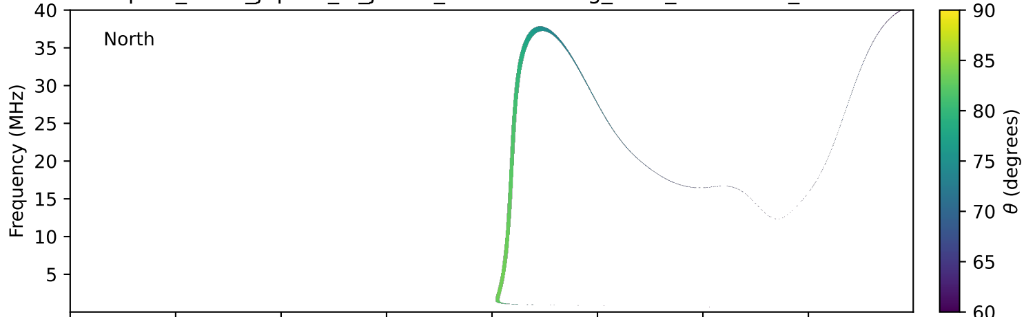
expres_earth_jupiter_io_jrm33_lossc-wid1deg_3kev_20161203_v11.cdf
