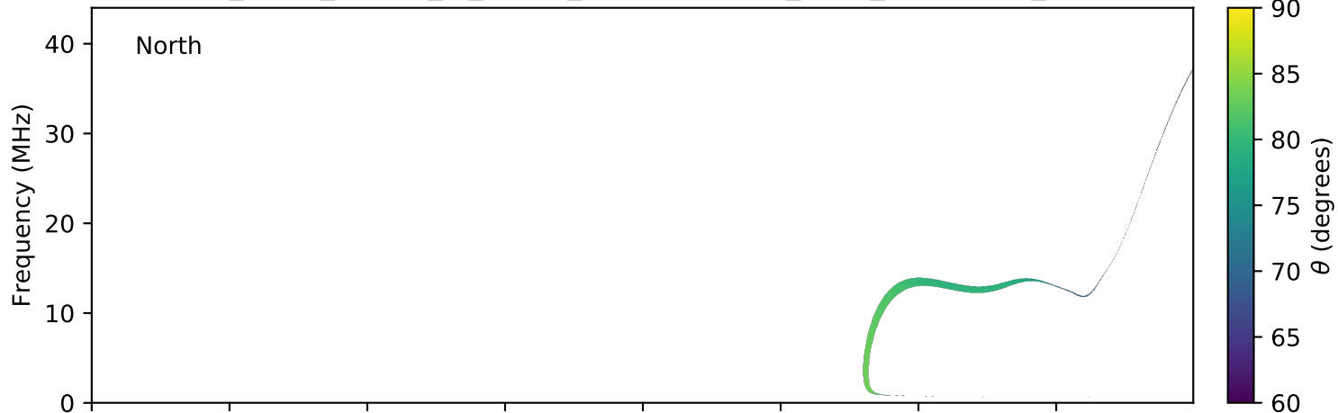
expres_earth_jupiter_io_jrm09_lossc-wid1deg_3kev_20161224_v01.cdf
