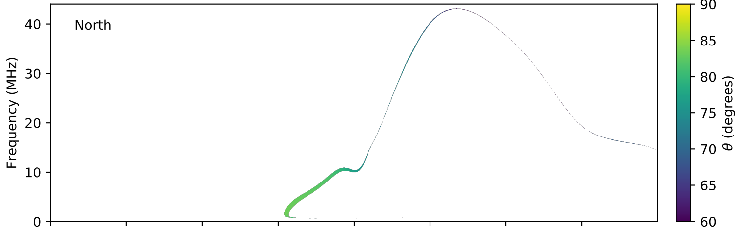
expres_earth_jupiter_io_jrm09_lossc-wid1deg_3kev_20161219_v01.cdf
