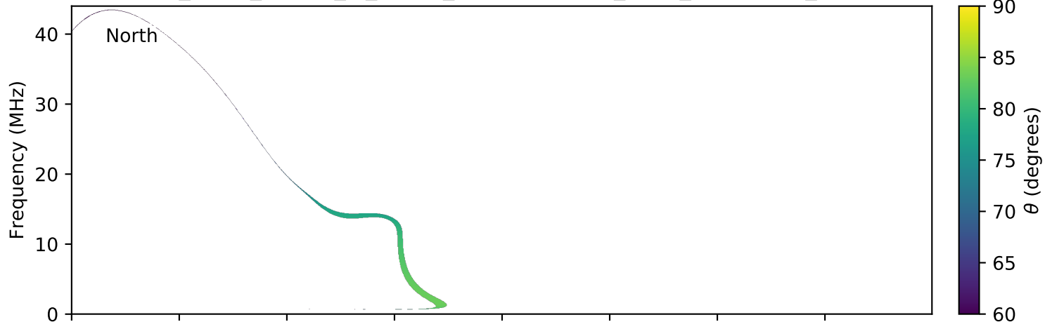
expres_earth_jupiter_io_jrm09_lossc-wid1deg_3kev_20161218_v01.cdf
