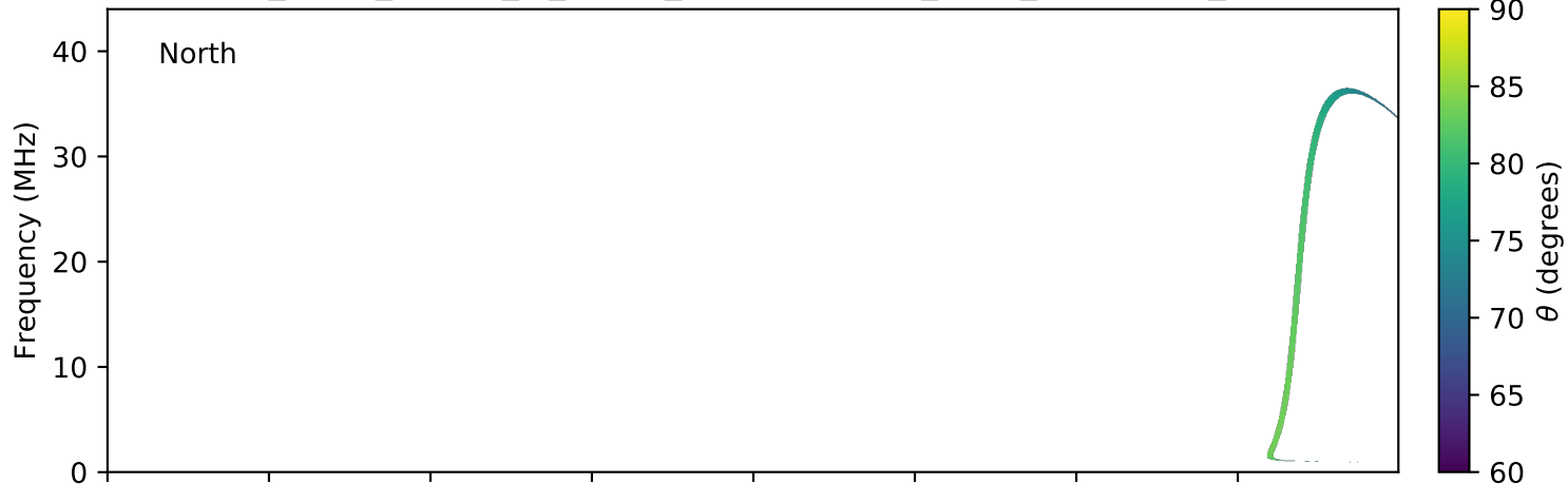
expres_earth_jupiter_io_jrm09_lossc-wid1deg_3kev_20161215_v01.cdf
