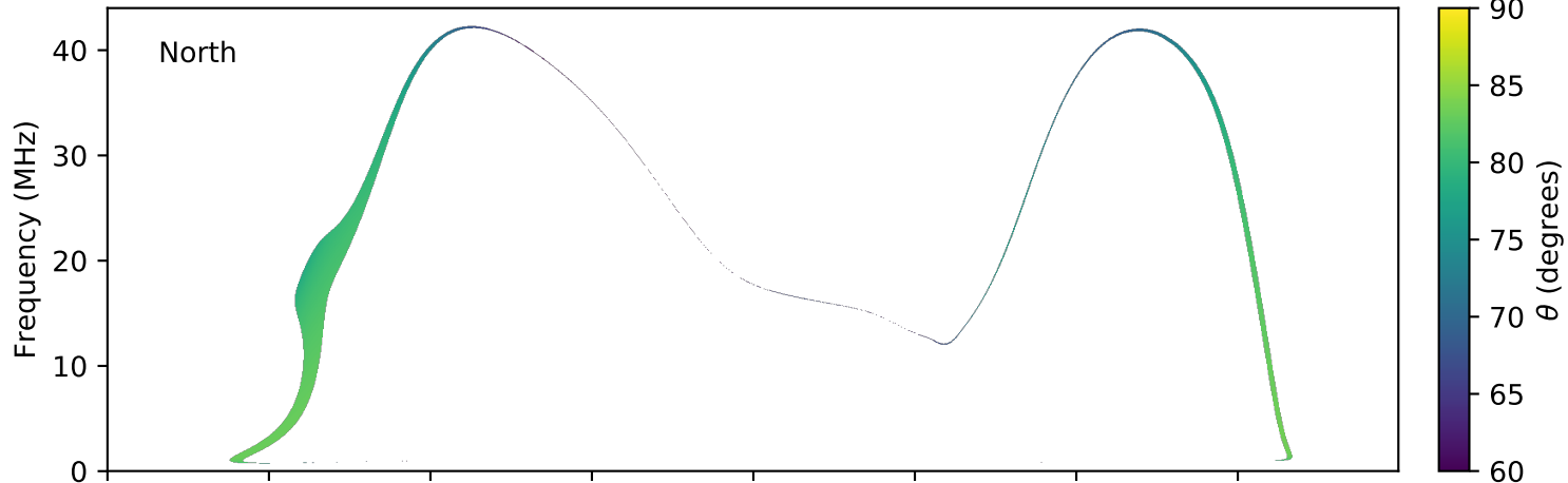
expres_earth_jupiter_io_jrm09_lossc-wid1deg_3kev_20161214_v01.cdf
